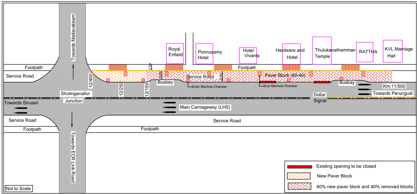
Line SKetch SHowing the location of rectification of service road from km:11/550 to 12/400 on RHS at OMR
