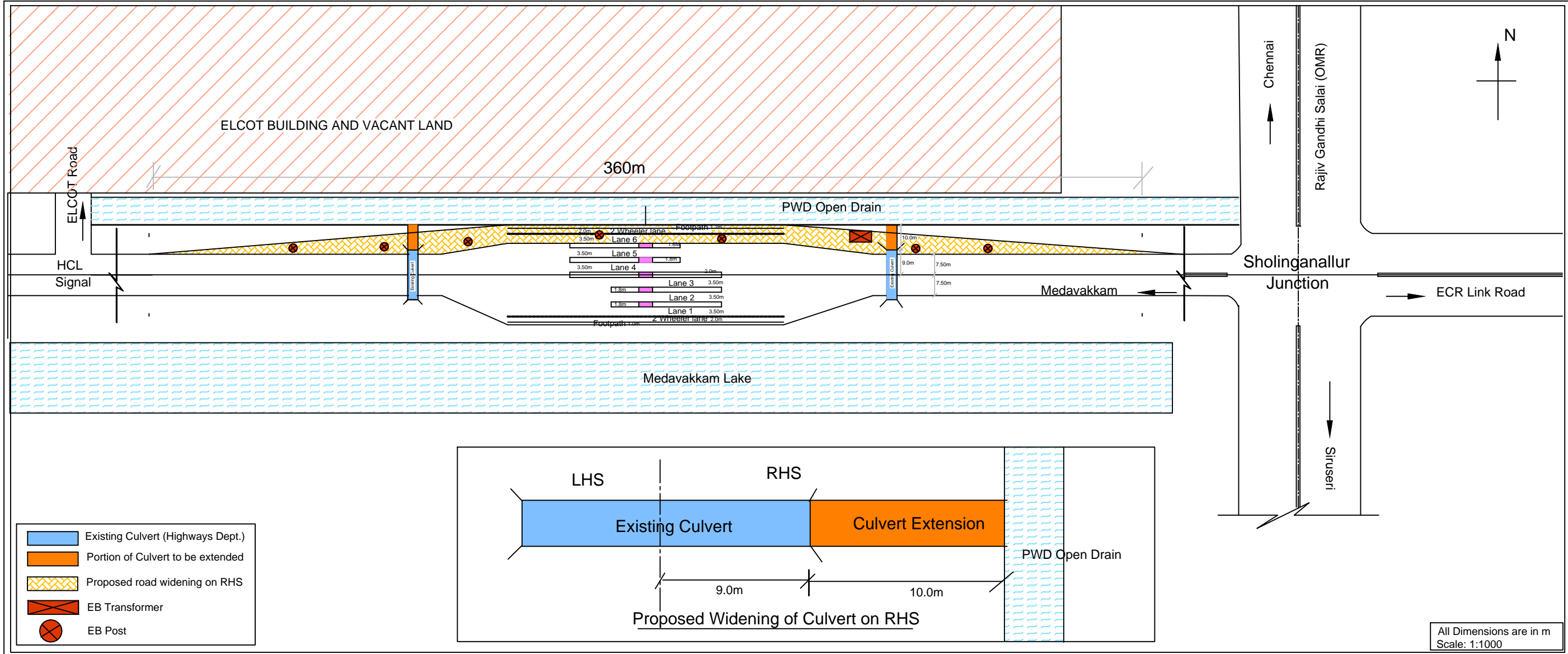
Line Skecth showing the details of the proposed culvert widening and road widening on RHS at Medavakkam Plaza, Medavakkam Road, OMR
