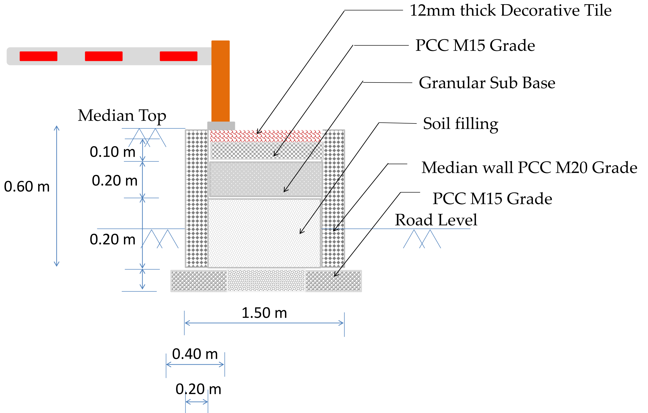
MEDIAN CROSS SECTION AT THORAIPAKKAM AND MEDAVAKKAM TOLL PLAZA
