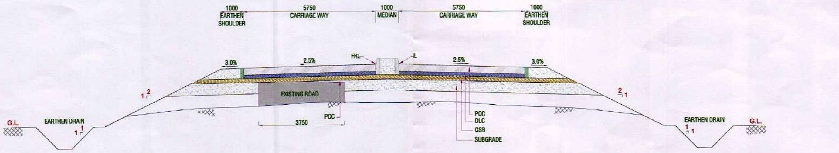
TYPICAL CROSS SECTION AT- 0+000 TO 0+700
