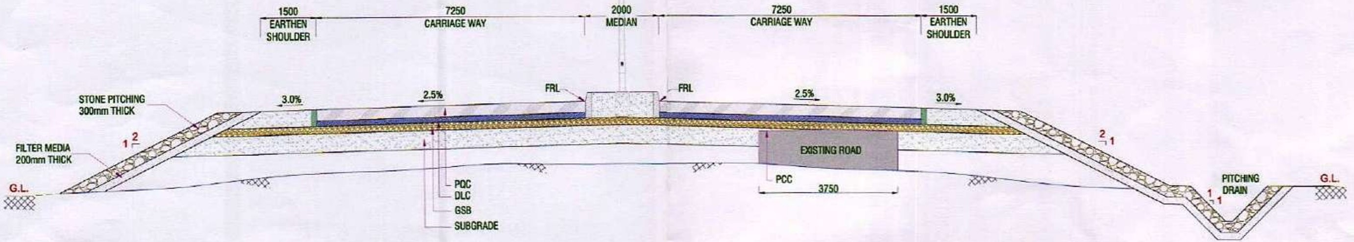
TYPICAL CROSS SECTION AT- 0+000 TO 2+100
