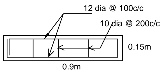
TNEB duct precast cover slab
