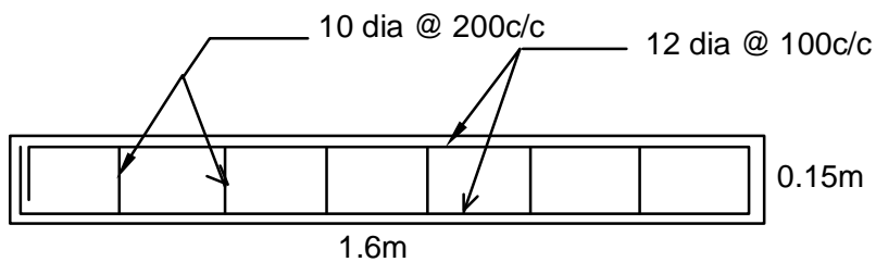
SD/EB Duct Precast Cover Slab
