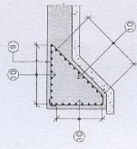
R.C. DETAILS
