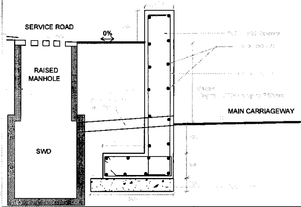
(b). Level difference between the MCW and Service Road > 300\text{mm}
