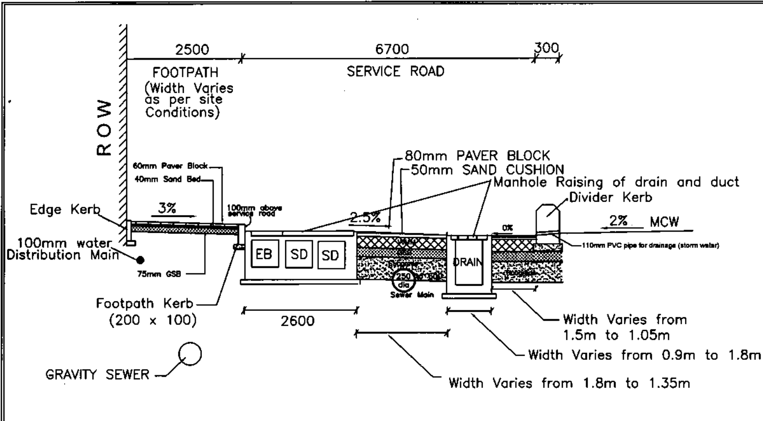
TYPICAL CROSS SECTION FROM CH: 22.500 TO CH:26.500 on RHS
