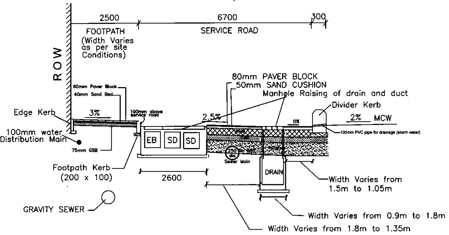
TYPICAL CROSS SECTION FROM CH: 22.500 TO CH:26.500 on RHS
